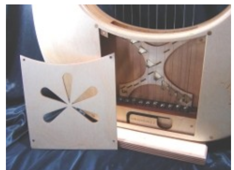
Rear view with the magnetic “Hatch Panel” removed to show an easy access for replacing any string.
